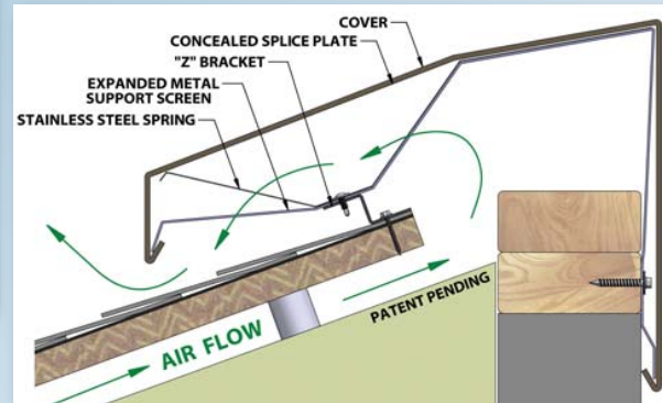
Sloped Roof Meets Vertical Wall Version
