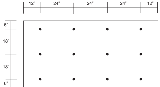
12 Fasteners/Bd.
