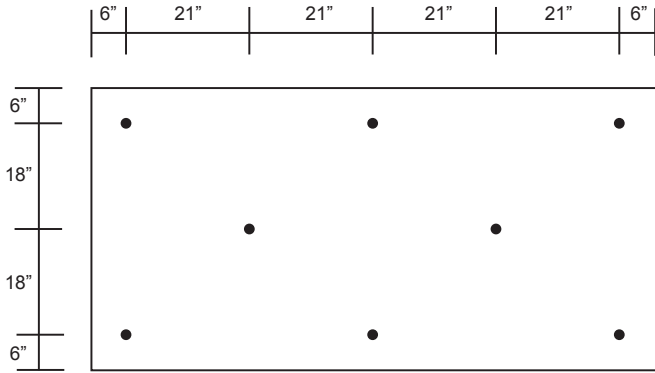
8 Fasteners/Bd.
